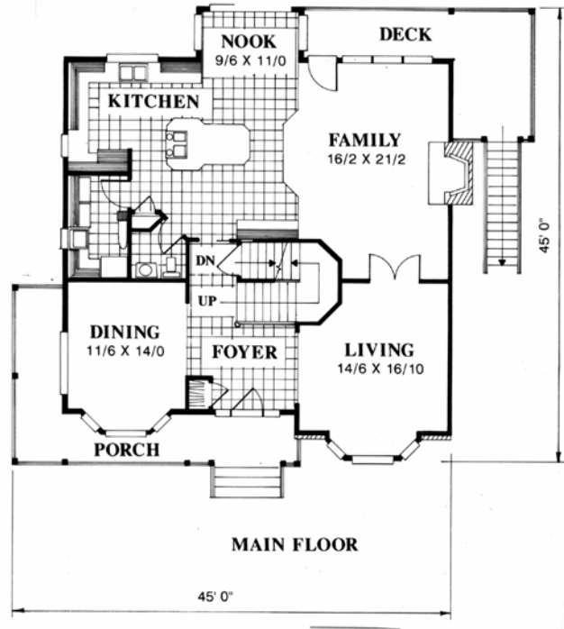
Optional Elevation and revision to plan M-3410 for Carlson Custom Homes.
