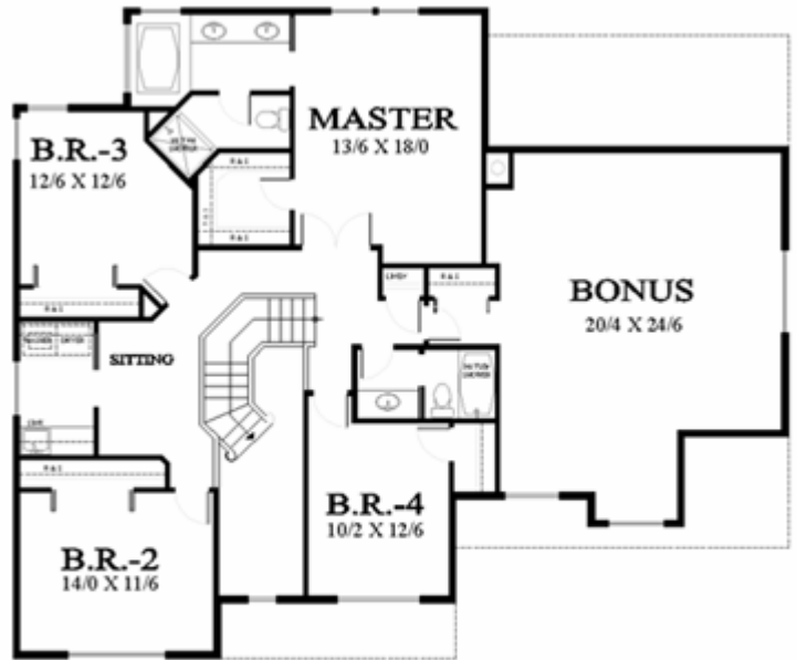
UPPER FLOOR PLAN - 1332 SQ. FT. (BONUS - 520 SQ. FT.)
