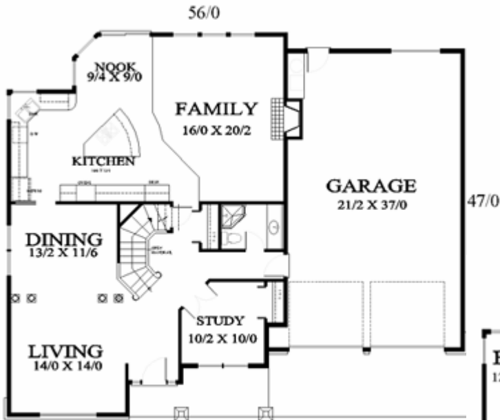
MAIN FLOOR PLAN - 1438 SQ. FT. (GARAGE - 805 SQ. FT.)
