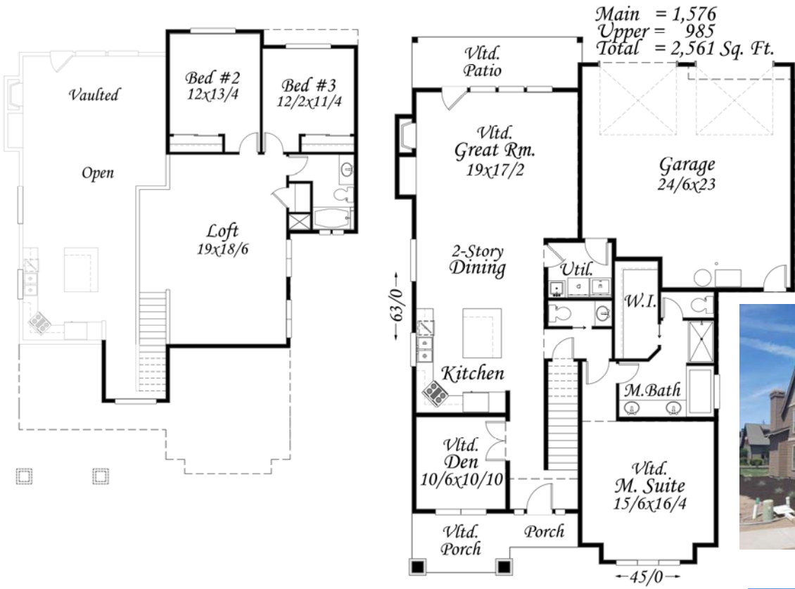
M-2561-GFHS 1576 sq. ft main 985 sq. ft upper 45/0 x 63/0
